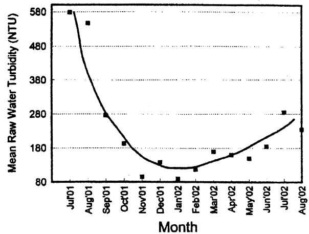
Figure -1 : Monthly variation of Mean Raw Water Turbidity
