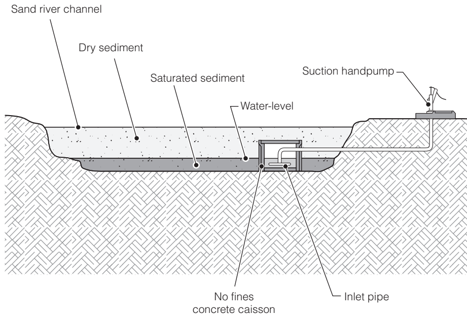
Figure 4.10. Riverbed caisson
