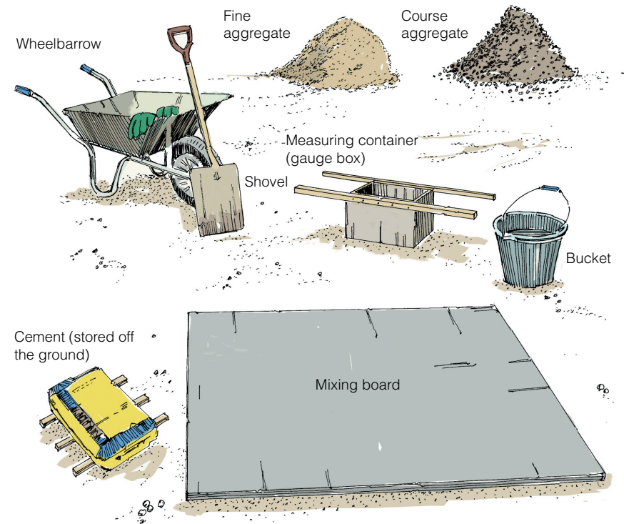
Figure 7. Materials and equipment required for handmixing concrete
