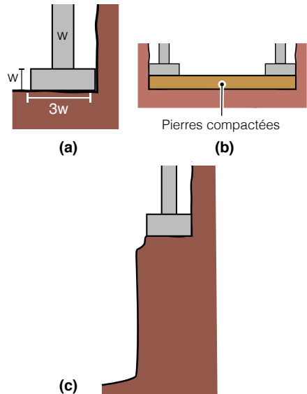
Figure 7. Fondations
